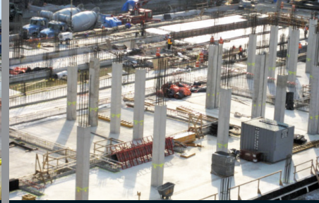
Croton UV Water Treatment Plant, USA
